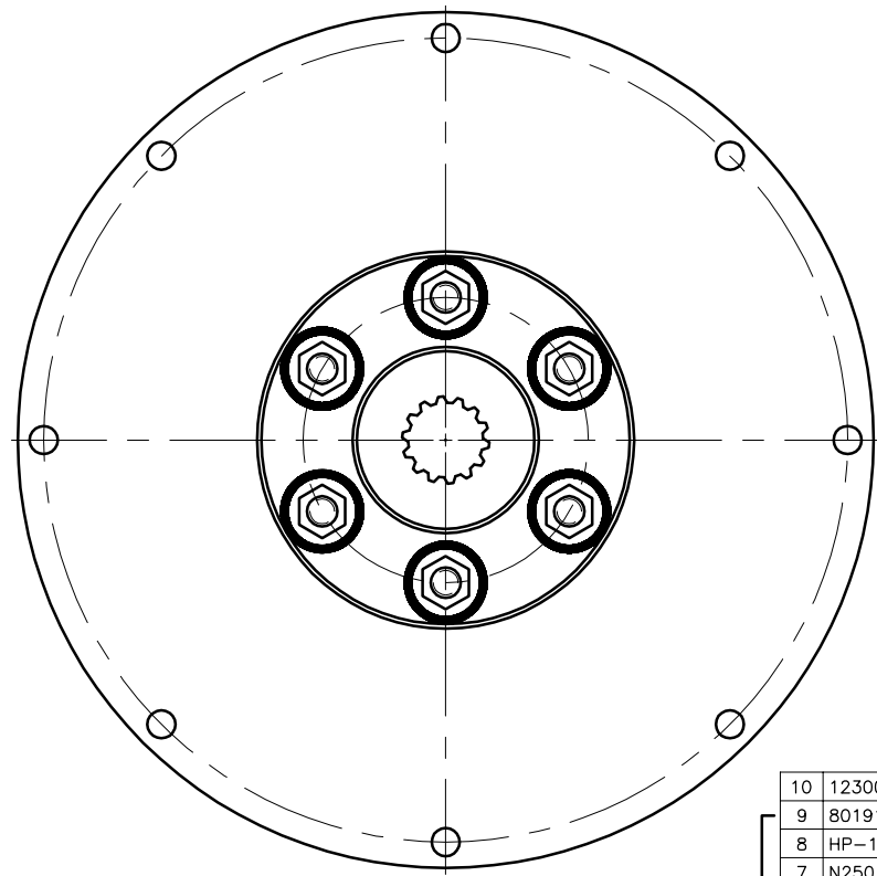
COUPLING ASS'Y #125345
