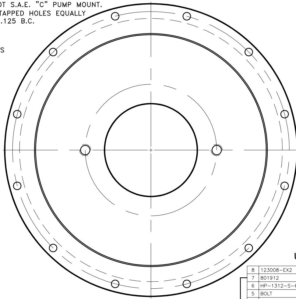
COUPLING ASS'Y #123040
