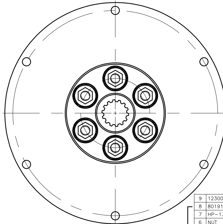
COUPLING ASS'Y #123316
