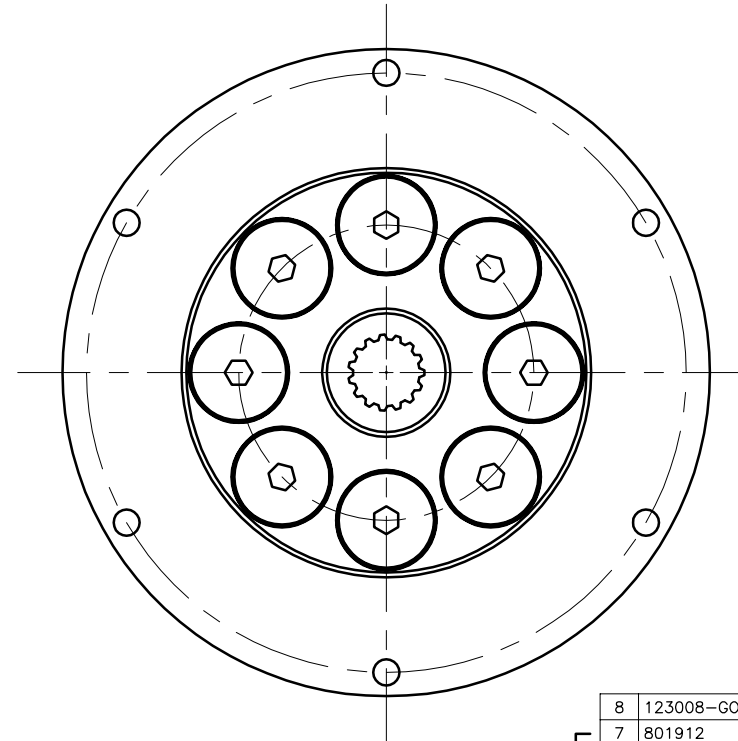
COUPLING ASS'Y #124418
