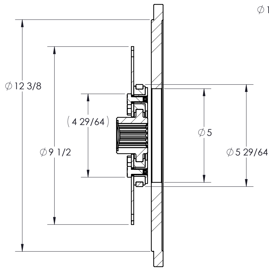
SECTION B-B
