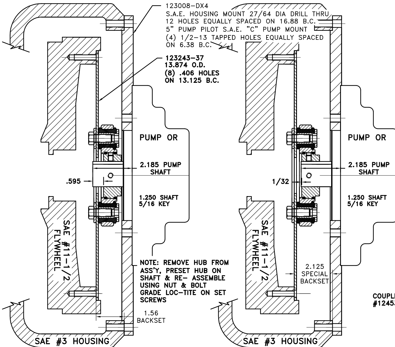
STANDARD SAE BACKSET
