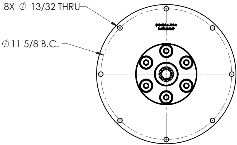
COUPLING FRONT VIEW
