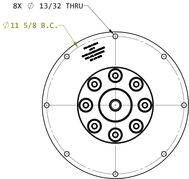
COUPLING FRONT VIEW
