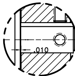
1.50 SHAFT LENGTH
