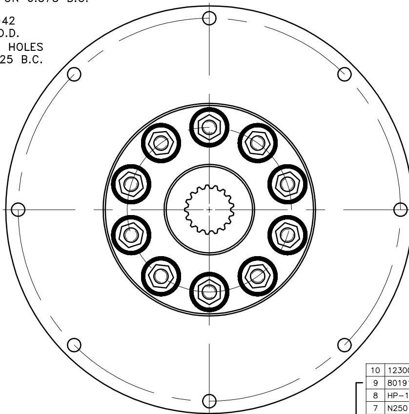
COUPLING ASS'Y #125880
