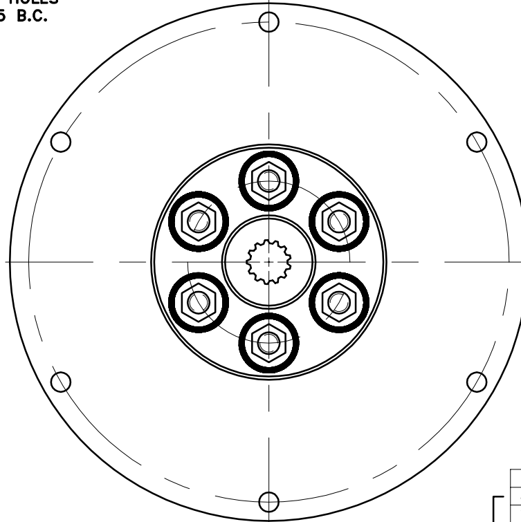
COUPLING ASS'Y #123294
