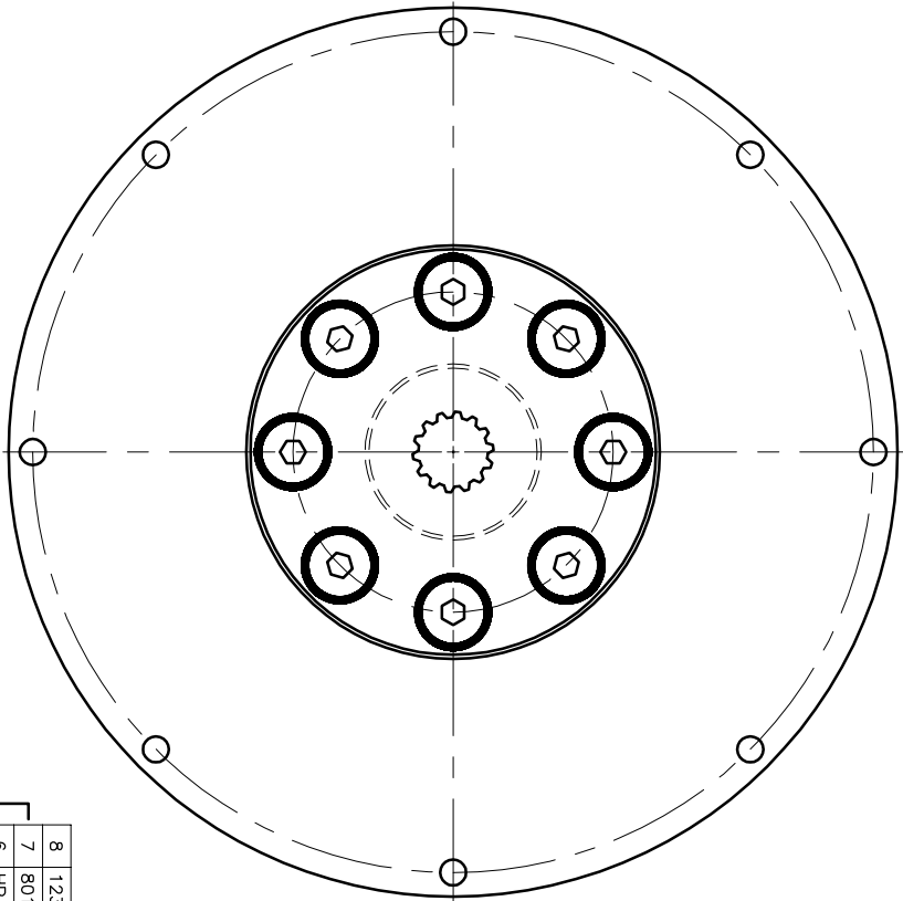
COUPLING ASS'Y - #123735
