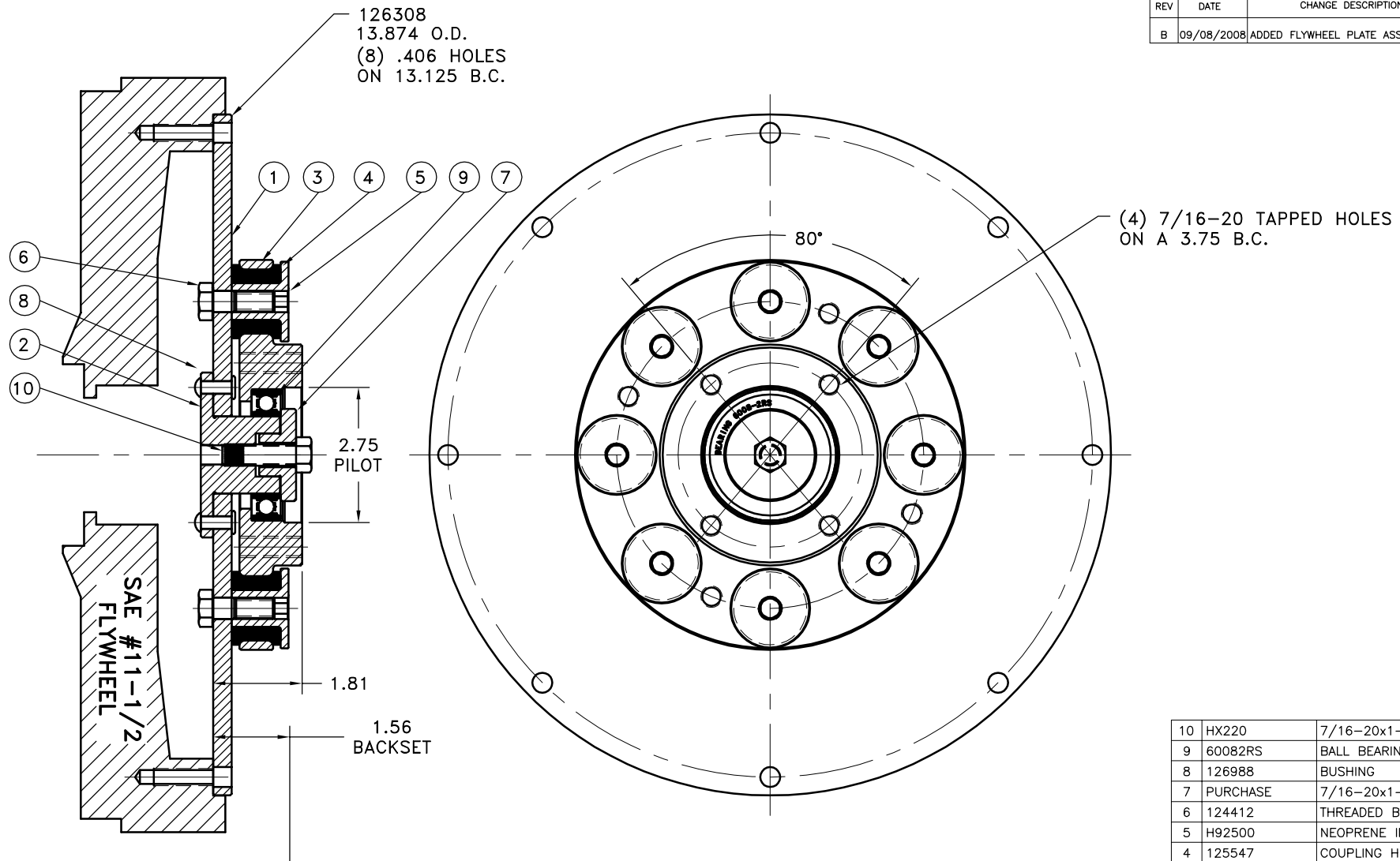
FLYWHEEL PLATE ASS'Y #129183
