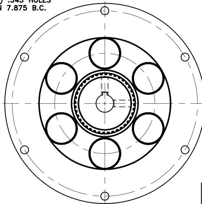
COUPLING ASS'Y #125204
