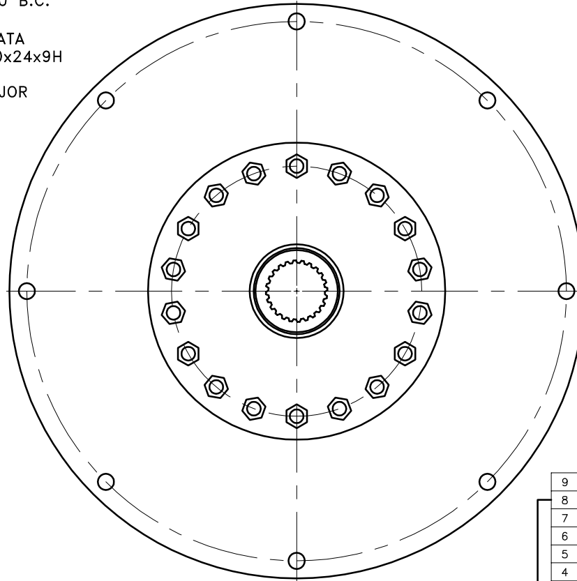
COUPLING ASS'Y #126543
