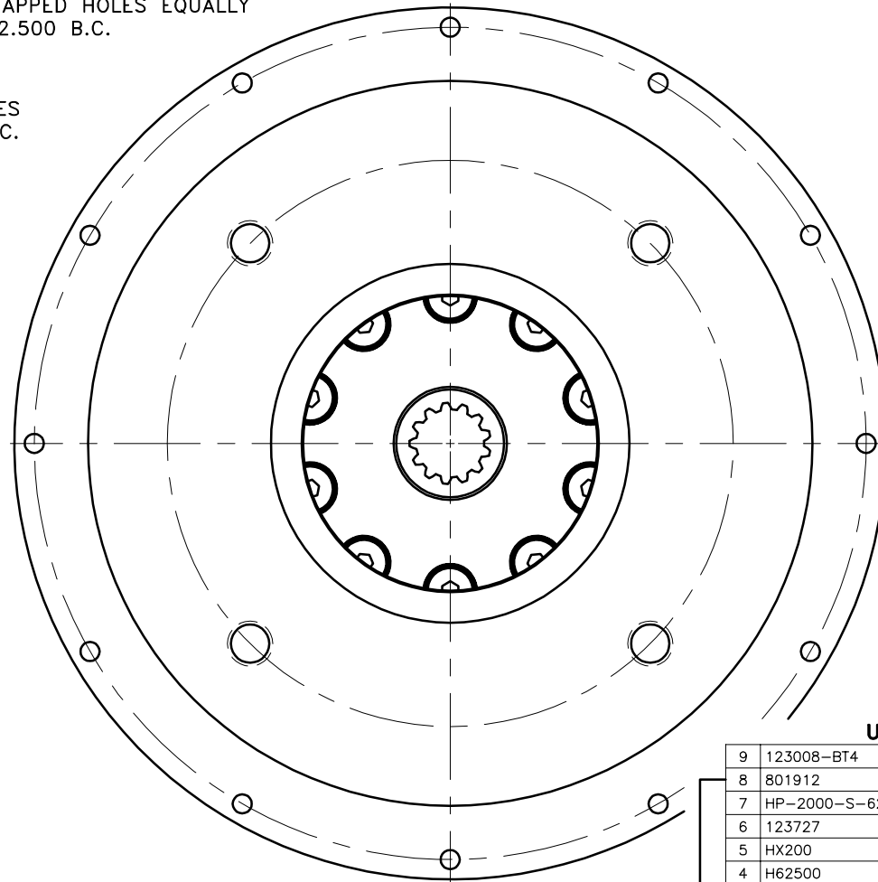
COUPLING ASS'Y #123433
