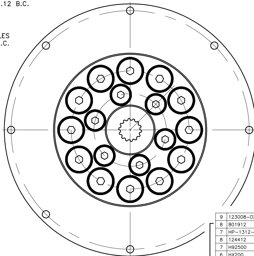
COUPLING ASS'Y #127011
