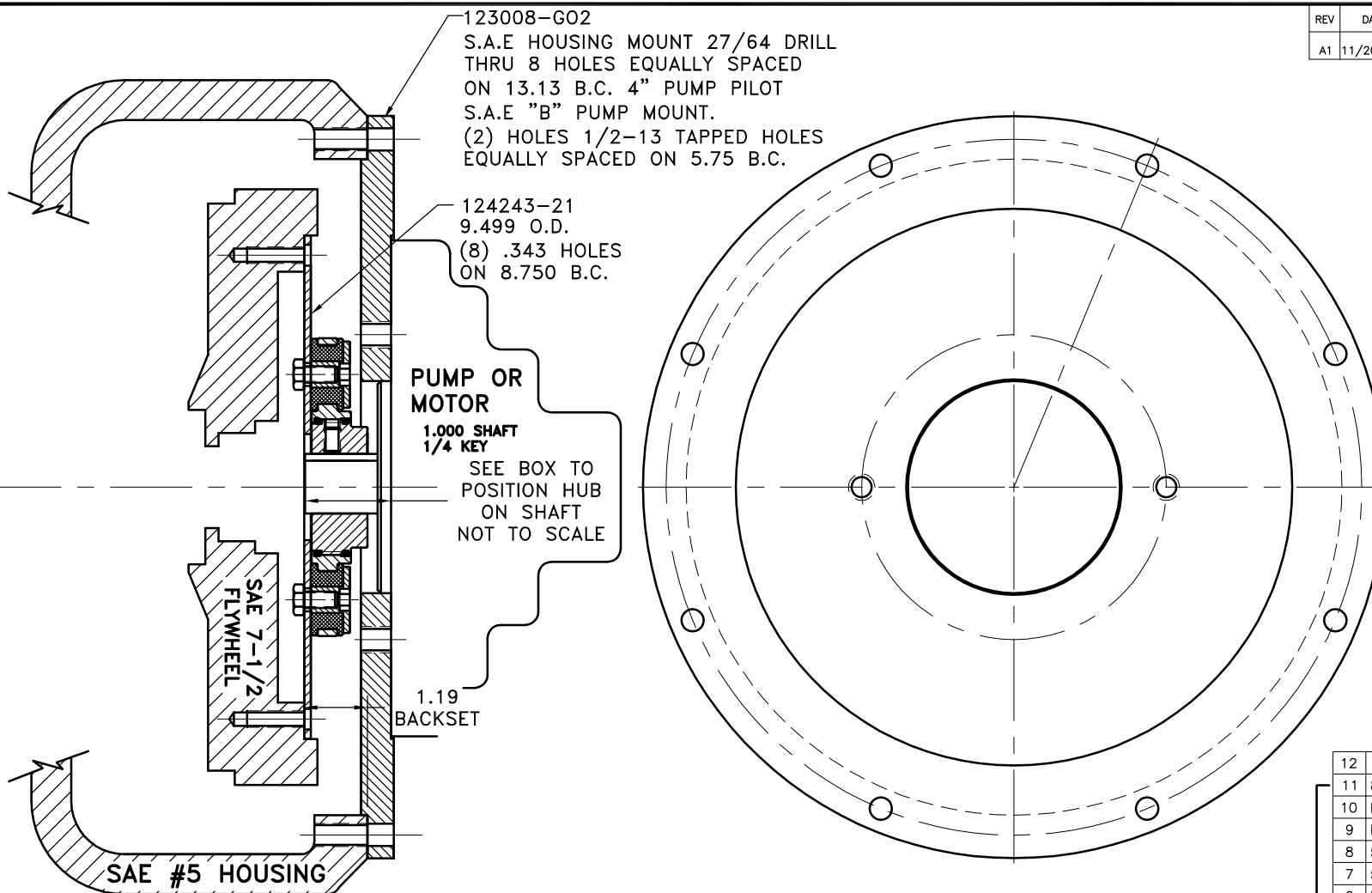
COUPLING ASS'Y #124404
