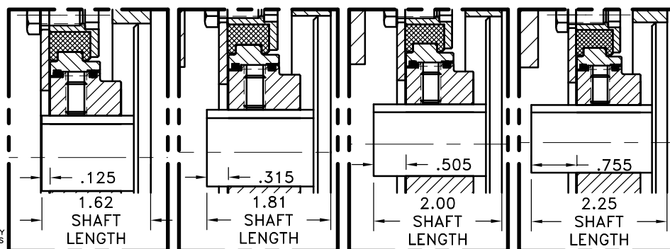
COUPLING ASS'Y #124404
