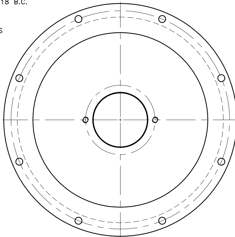
COUPLING ASS'Y #125204
