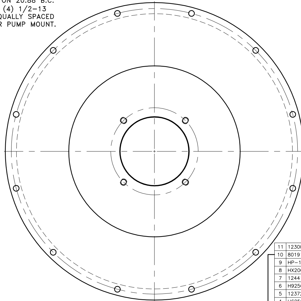
COUPLING ASS'Y 127673
