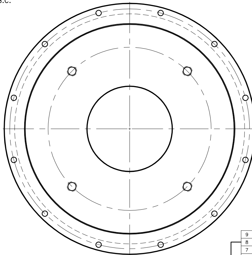
COUPLING ASS'Y #127303
