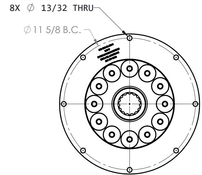
FLYWHEEL COUPLING FRONT VIEW
