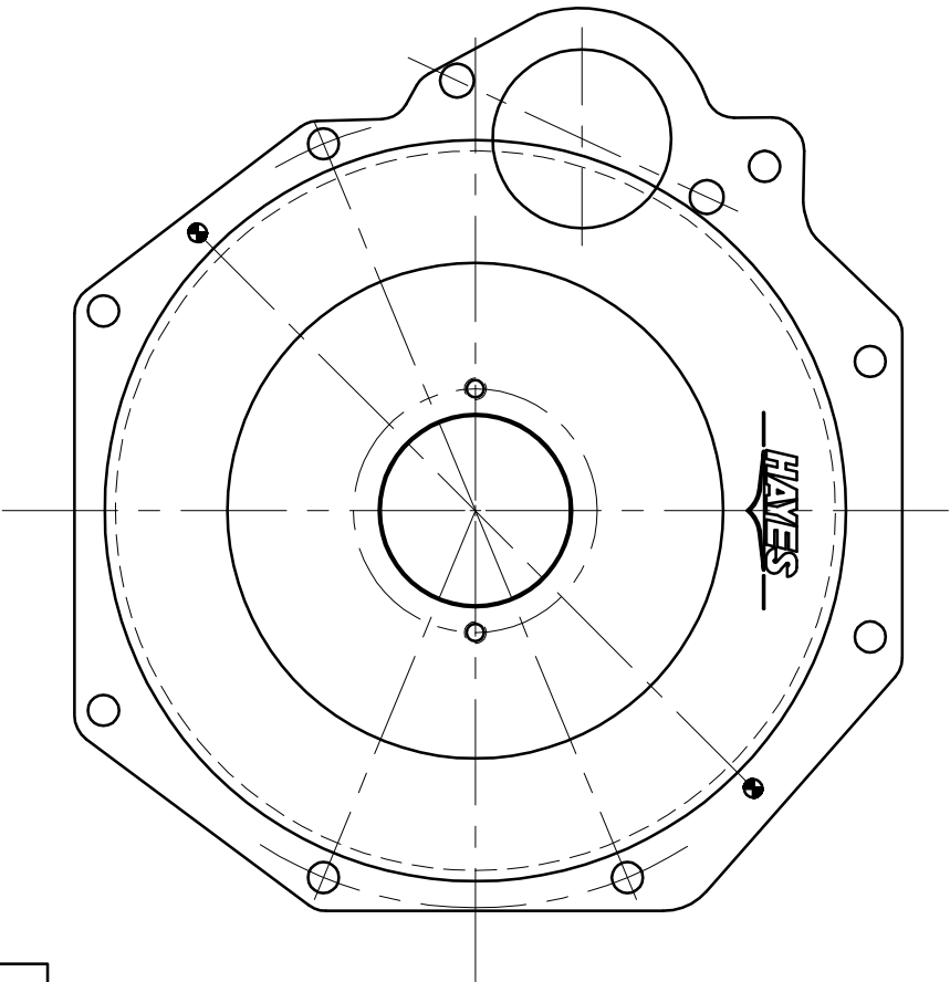
COUPLING ASSY #127669-
