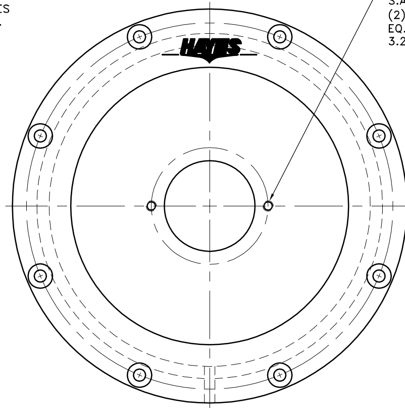
COUPLING ASS'Y #123272-13
