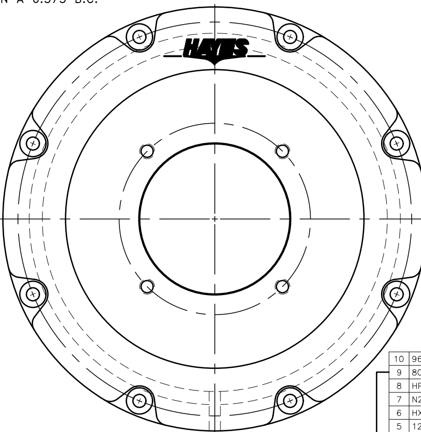
COUPLING ASS'Y #125408
