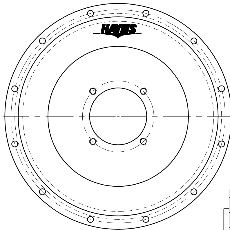
COUPLING ASS'Y #125208
